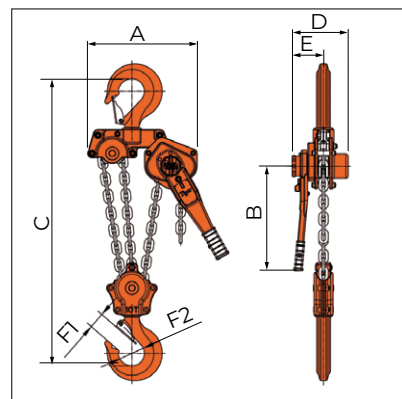
PLH-1000 / 10,0t
