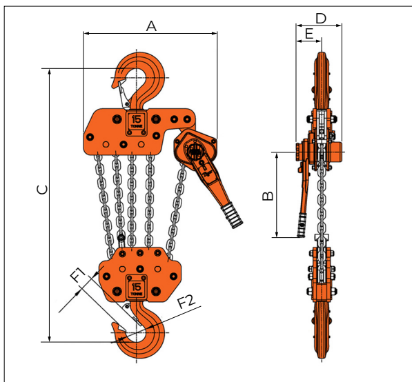
PLH-1500 / 15,0t
