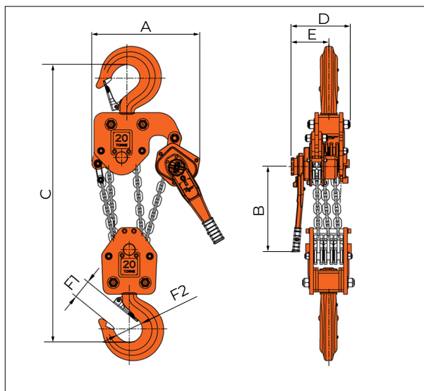
PLH-2000 / 20,0t
