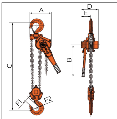
PLH-0630 / 6,0 / 6, t
