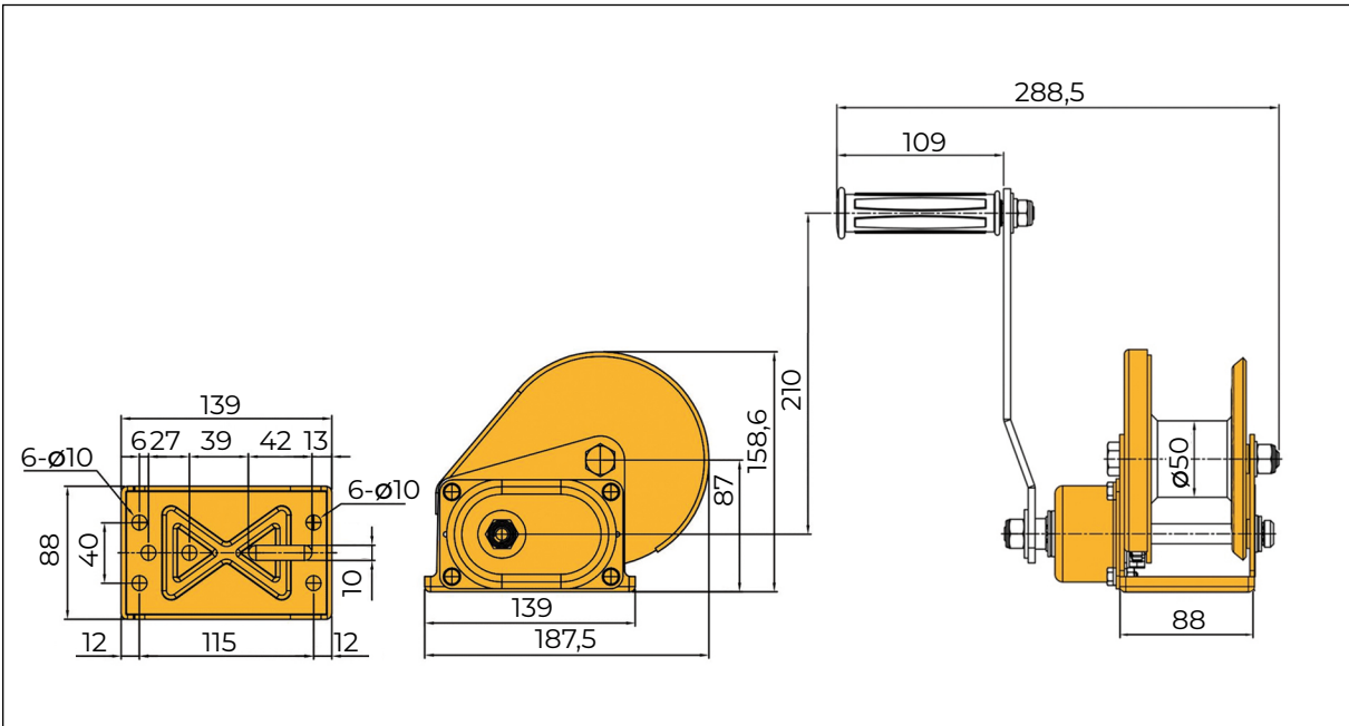
BHW-1200-N
