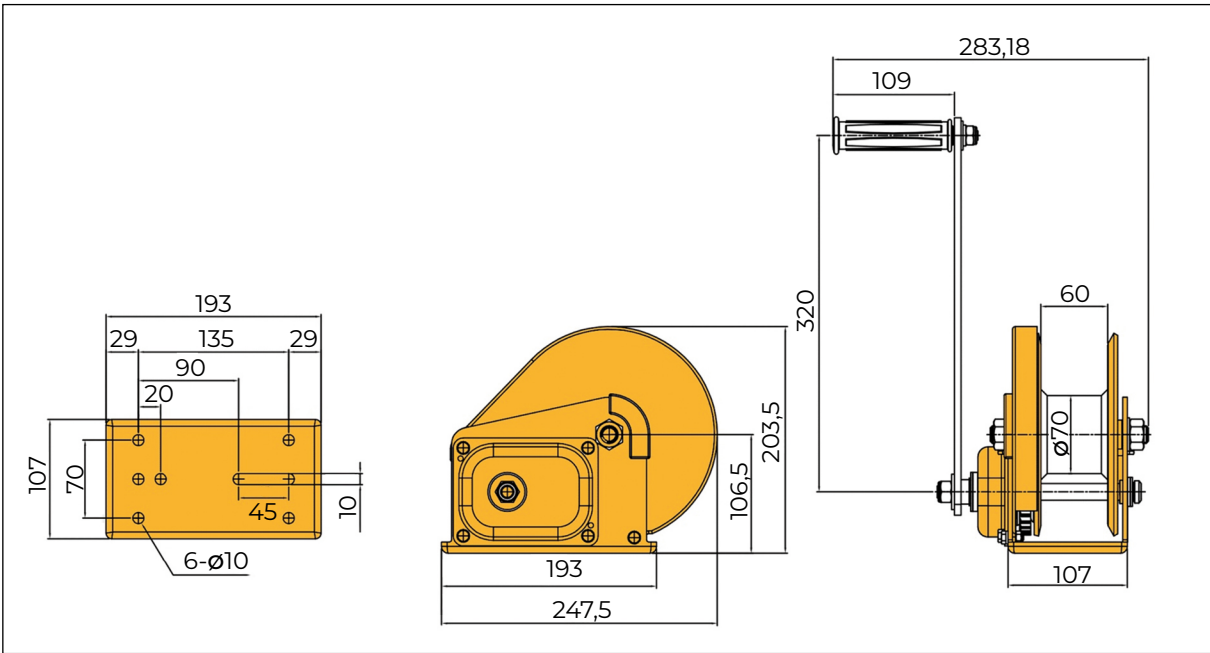
BHW-2600
